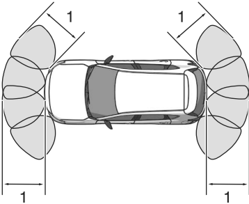
Detection ranges of ultrasonic sensors Vehicles with 360° View Monitor
